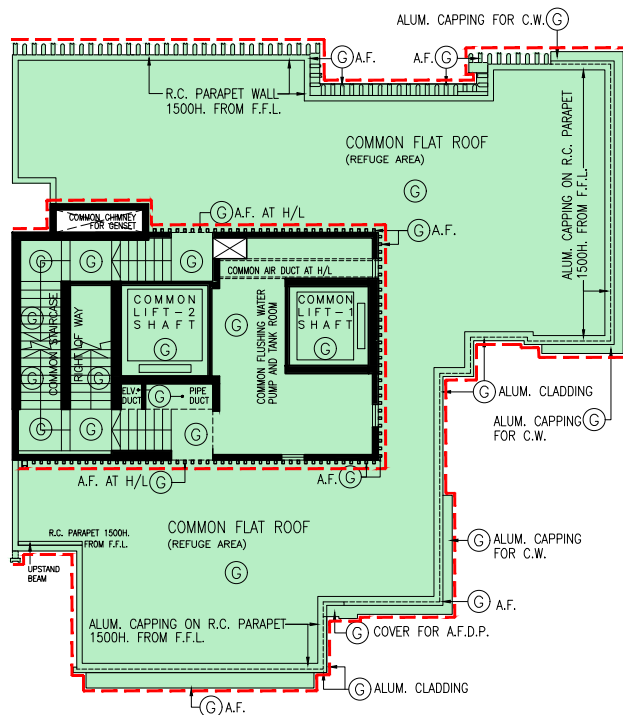
ROOF PLAN (FOR IDENTIFICATION PURPOSE ONLY) (NOT TO SCALE)
