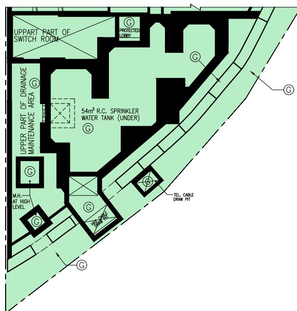
PART PLAN FOR UPPER LG1 FLOOR (FOR IDENTIFICATION PURPOSE ONLY) (NOT TO SCALE)
