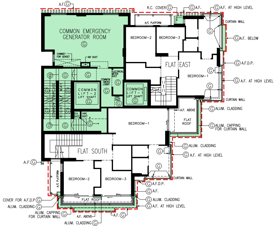
29TH FLOOR PLAN (FOR IDENTIFICATION PURPOSE ONLY) (NOT TO SCALE)
