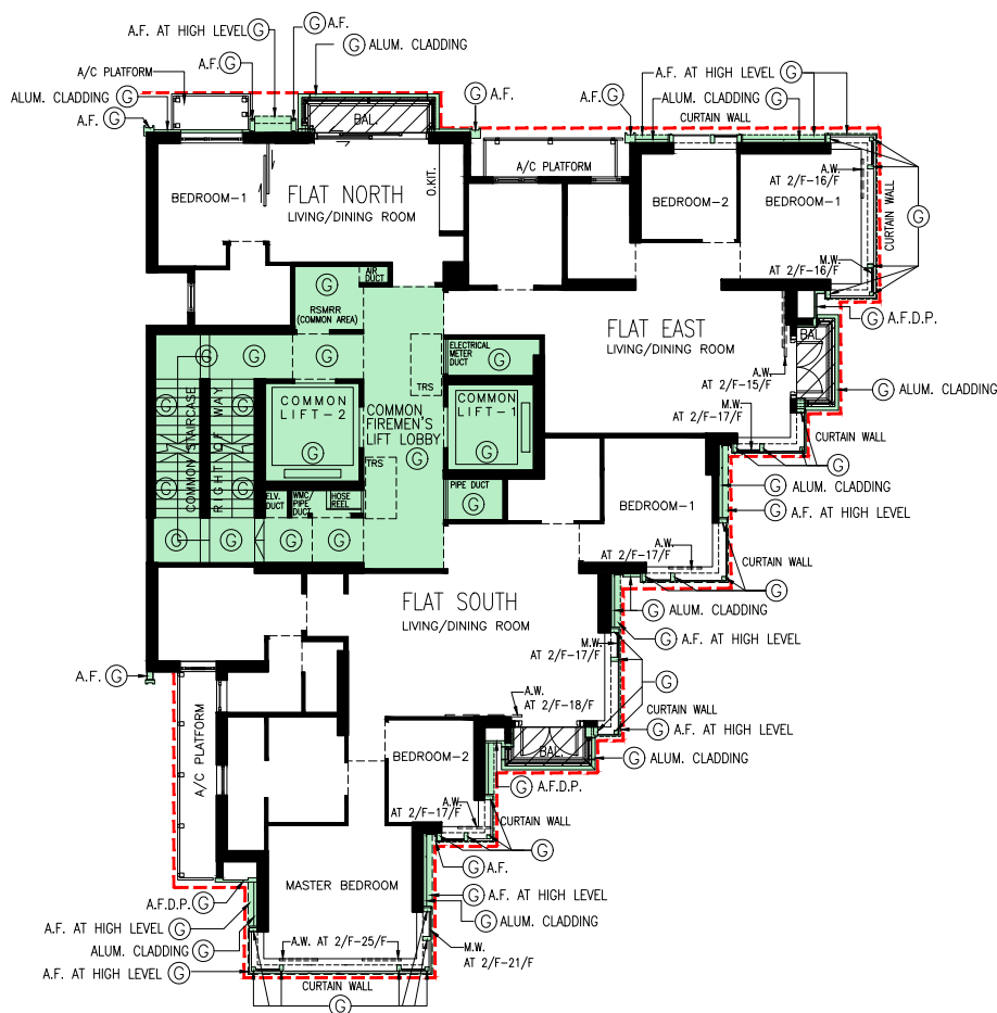
2ND-27TH FLOOR PLAN (FLOOR NUMBERING 4/F, 13/F, 14/F & 24/F OMITTED) (FOR IDENTIFICATION PURPOSE ONLY) (NOT TO SCALE)
