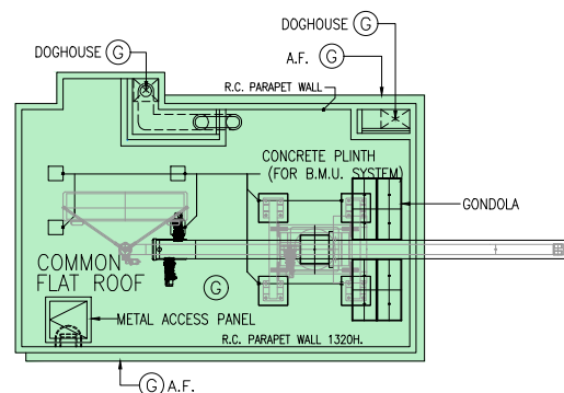
TOP ROOF PLAN (FOR IDENTIFICATION PURPOSE ONLY) (NOT TO SCALE)
