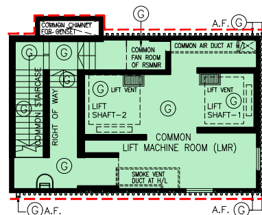
UPPER ROOF PLAN (FOR IDENTIFICATION PURPOSE ONLY) (NOT TO SCALE)
