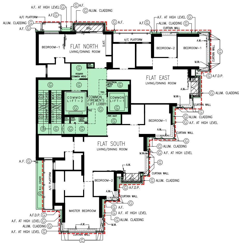
1ST FLOOR PLAN (FOR IDENTIFICATION PURPOSE ONLY) (NOT TO SCALE)
